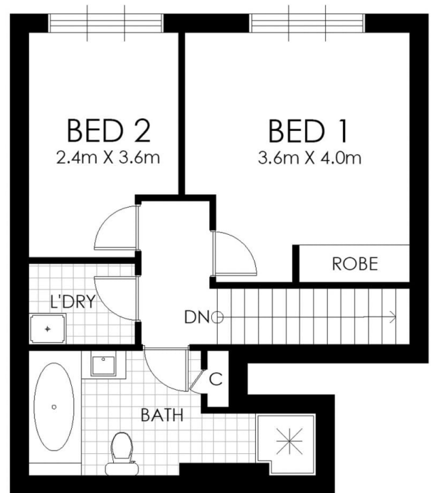
UPPER LEVEL
